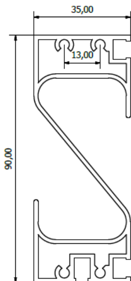
S-HANDGREEP (HR097)
