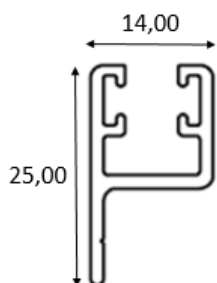
S-HANDGREEP (HR097)
